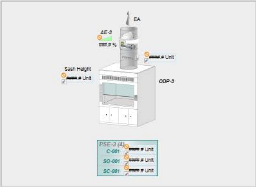
VAV-FHC MODULATING DAMER SERVES: FUME HOODS RM 220-1, 220-2, 220-3, 220-4 APP# 10741_FH
