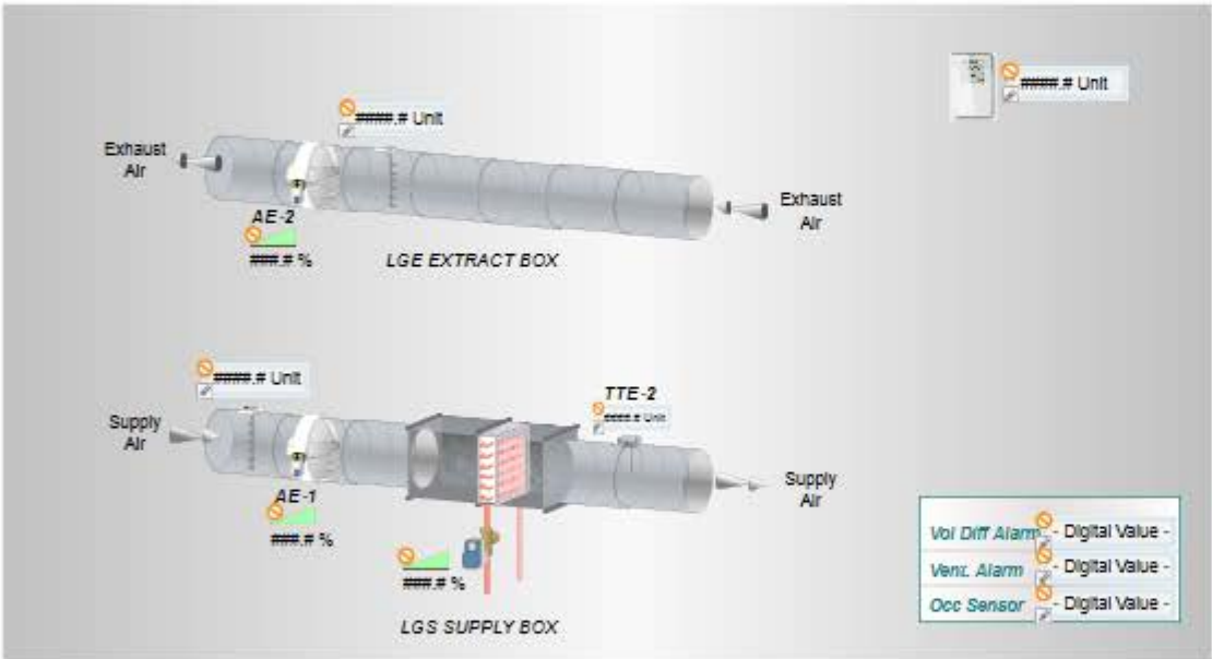
VAV-LRC - FAST ACT VAV W/ELEC RHT SERVES: LAB VAV SAV001B-000 APP# 10751_220
