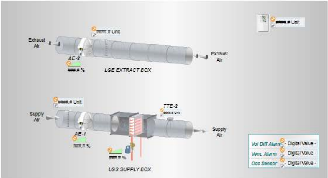
VAV-LRC - FAST ACT VAV W/ELEC RHT SERVES: LAB VAV SAV001B-004 APP# 10751_227
