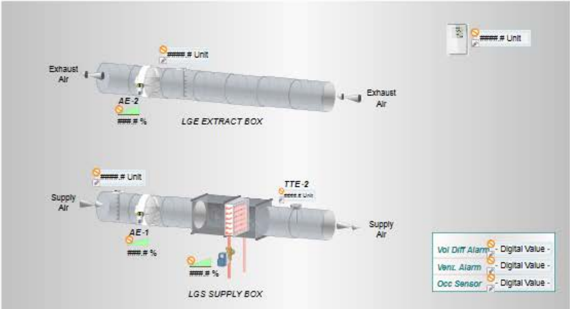
VAV-LRC - FAST ACT VAV W/ELEC RHT SERVES: FUME HOODS RM 212 APP# 10751_212
