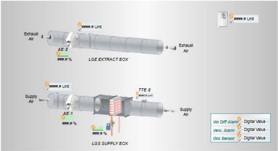
VAV-LRC - FAST ACT VAV W/ELEC RHT SERVES: LAB VAV SAV001B-001 APP# 10751_229
