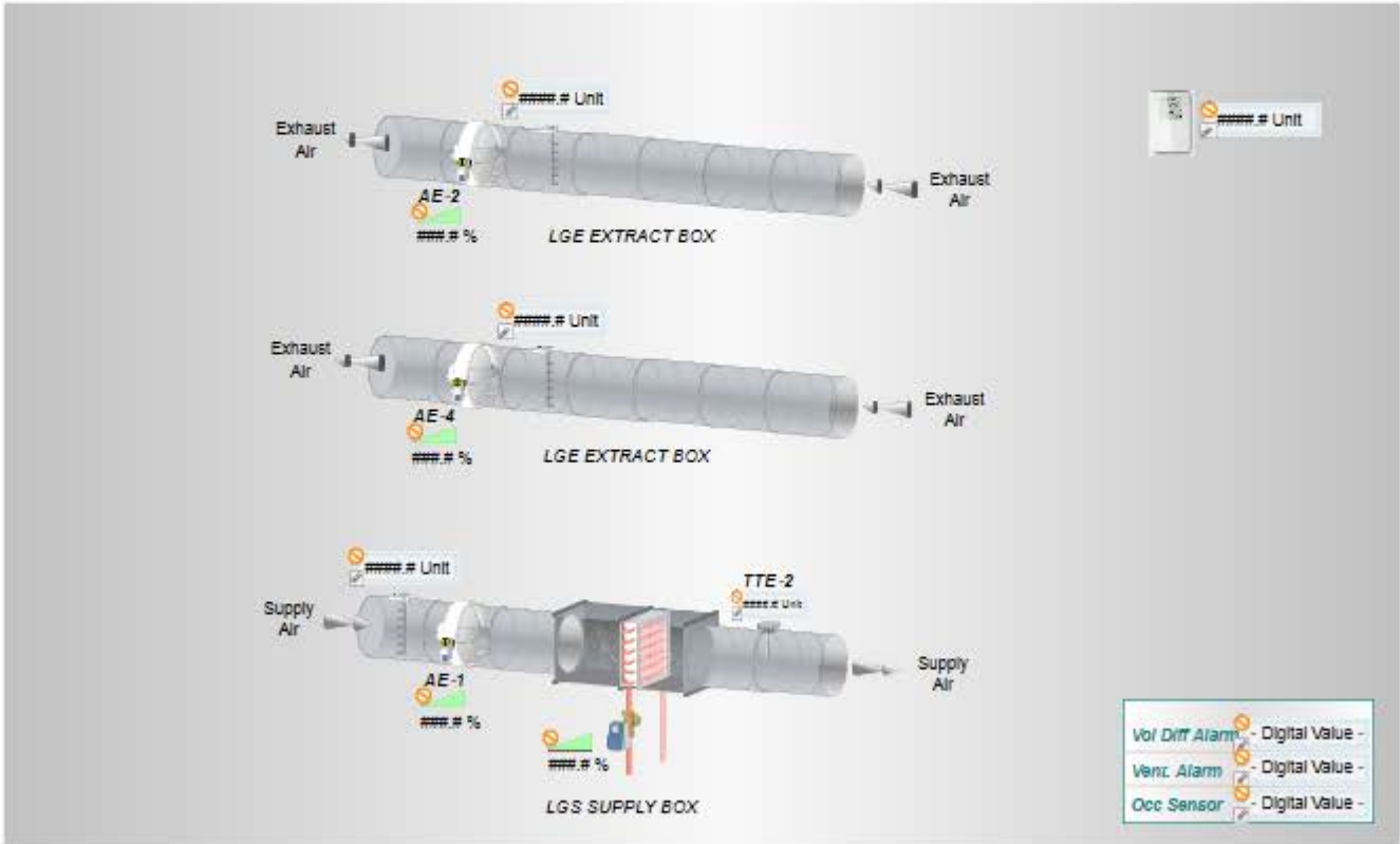
VAV-LRC - FAST ACT VAV W/ELEC RHT SERVES: LAB VAV SAV001B-008 APP#10751-213
