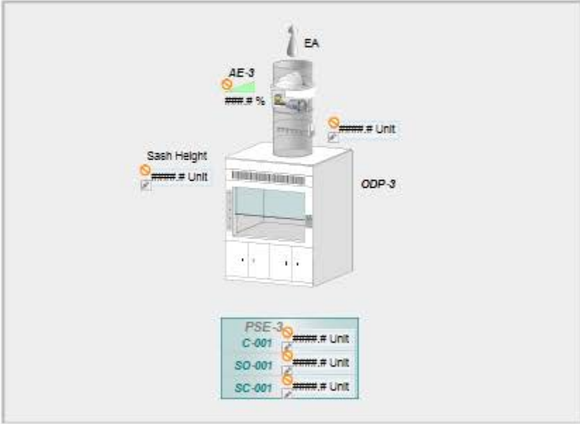
VAV-FHC MODULATING DAMER SERVES: FUME HOODS RM 227 APP# 10741_FH
