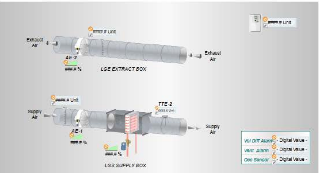
VAV-LRC - FAST ACT VAV W/ELEC RHT SERVES: LAB VAV SAV001B-003 APP# 10751_232
