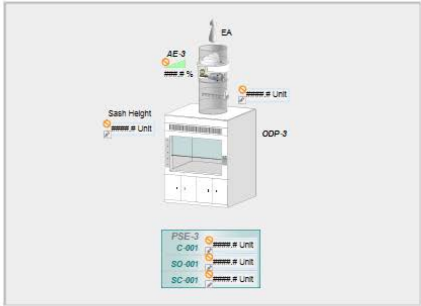
VAV-FHC MODULATING DAMER SERVES: FUME HOODS RM 230 APP# 10741_FH
