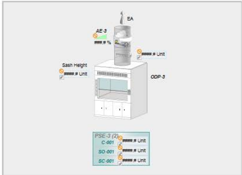
VAV-FHC MODULATING DAMER SERVES: FUME HOODS RM 232-1, 232-2 APP# 10741_FH
