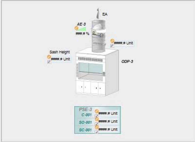
VAV-FHC MODULATING DAMPER SERVES: FUME HOODS RM 212 APP# 10741_FH
