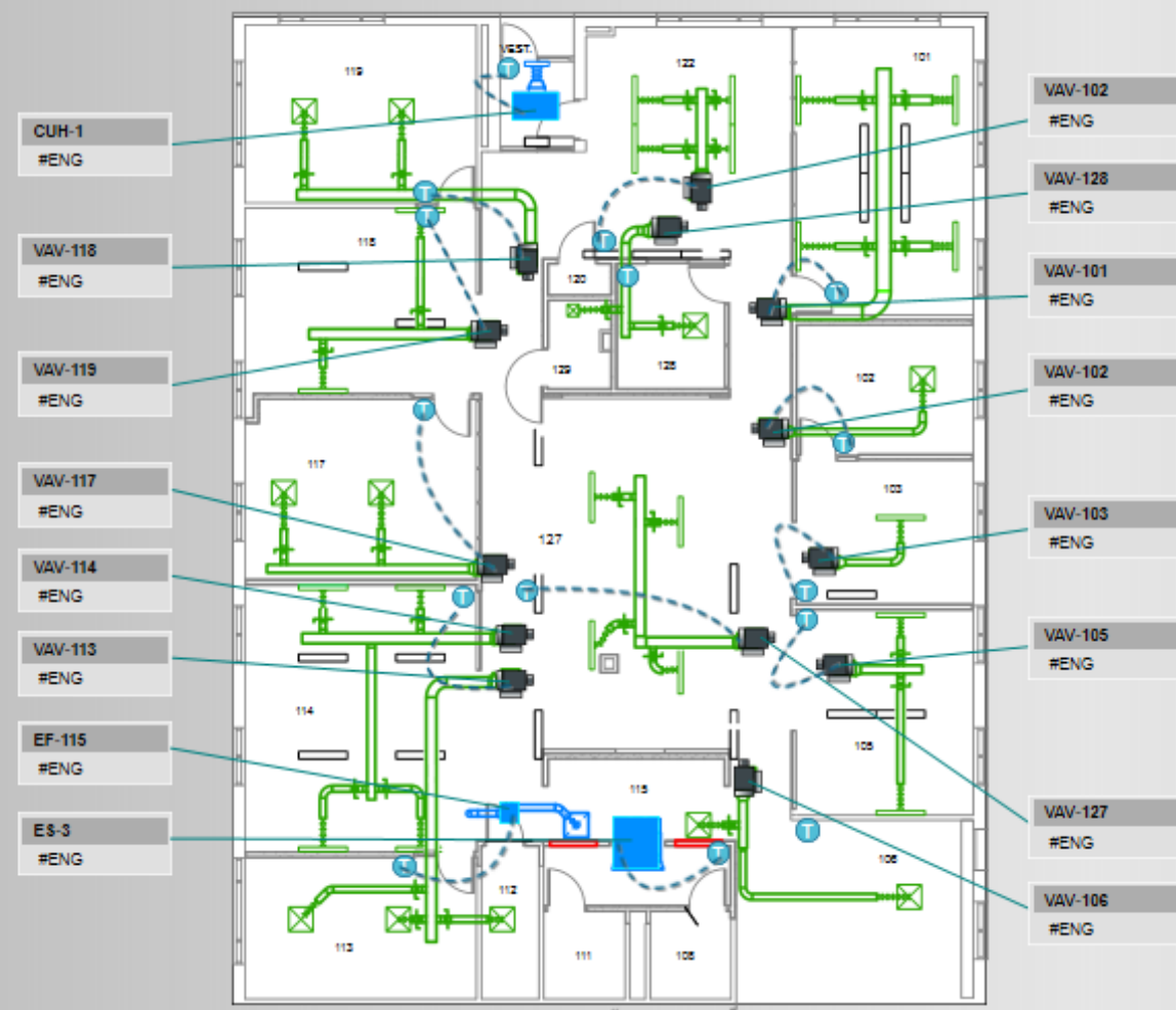
TOP VIEW
